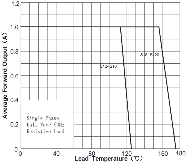
FIG1: Io-TL Curve
